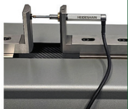
Checking of electronic probes
